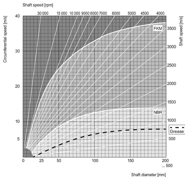
Limits for circumferential speed/speed depending on the diameter of the shaft and the material.
