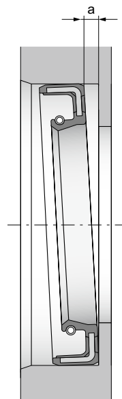
Representation of the skew
