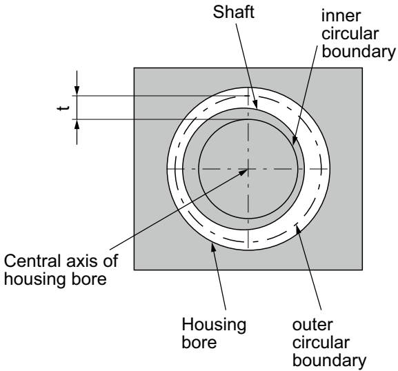
Illustration of the runout tolerance
