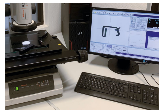
Profile cross-section inspection of a radial shaft seal
