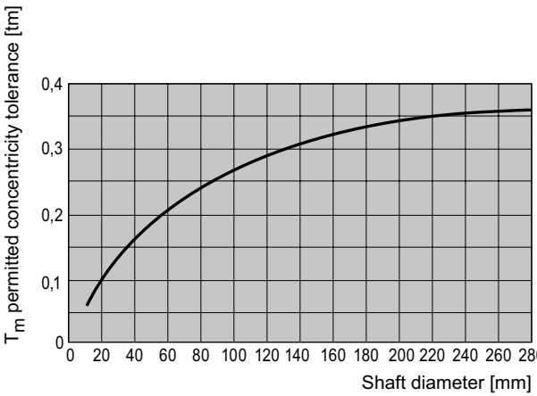
Permissible coaxiality tolerances of the shaft to the housing bore
