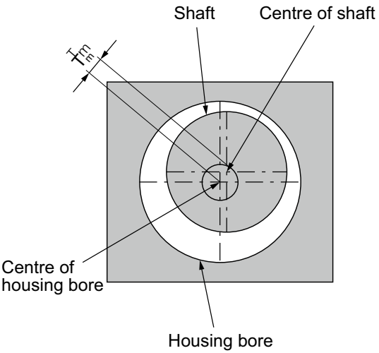
Illustration of the coaxiality tolerances
